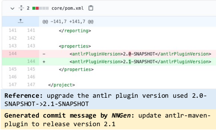
Fig. 2. An example of generated commit message with low automatic scores.
