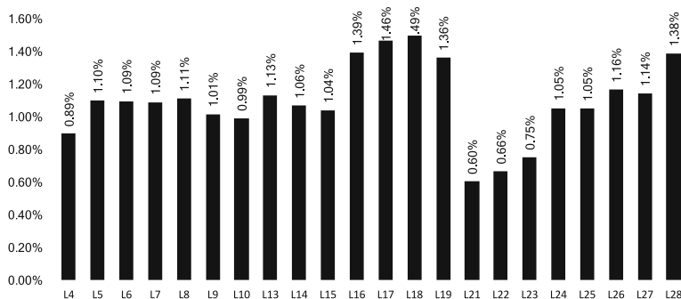
Fig. 4 Distribution of deprecated API rate. For each API level, all its deprecated APIs, including the ones that are deprecated in previous levels, are considered
