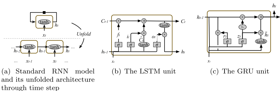
Fig. 1 An illustration of basic RNN, LSTM and GRU
