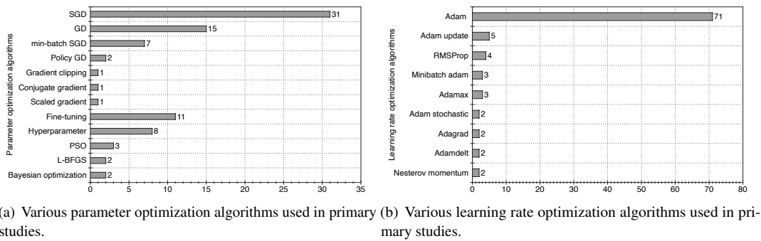
Fig. 4. Distribution of optimizers used in primary studies.
